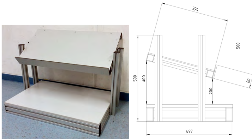
(a) A shelf with two levels and uniform colored surfaces. (b) Technical draw of shelf configuration.
